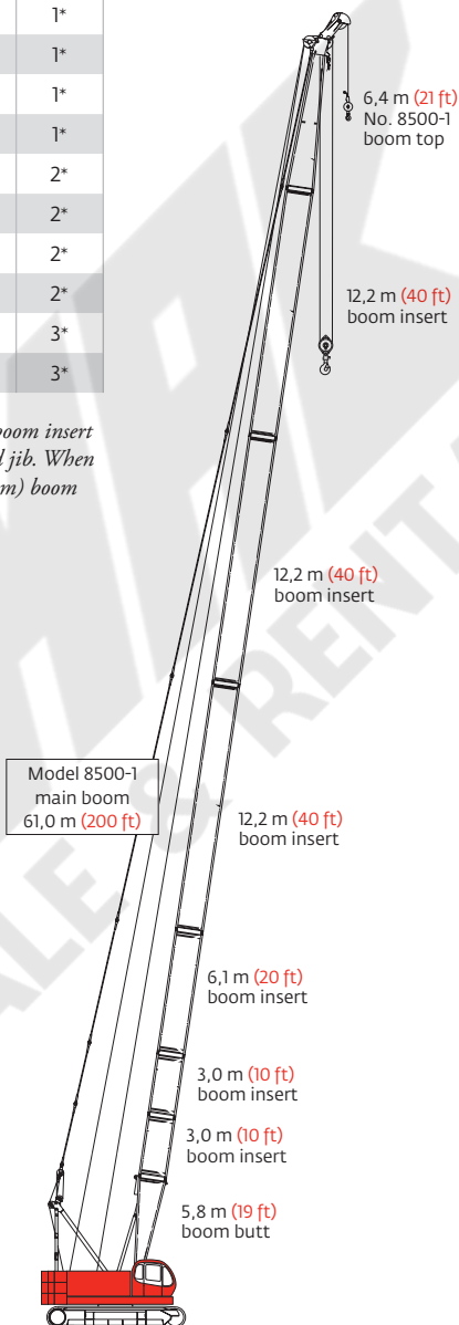
Model 8500-1 Main boom 61,0 m (200 ft)
