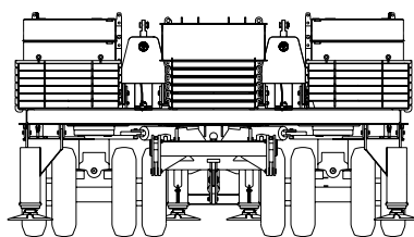
Counterweight arrangement
