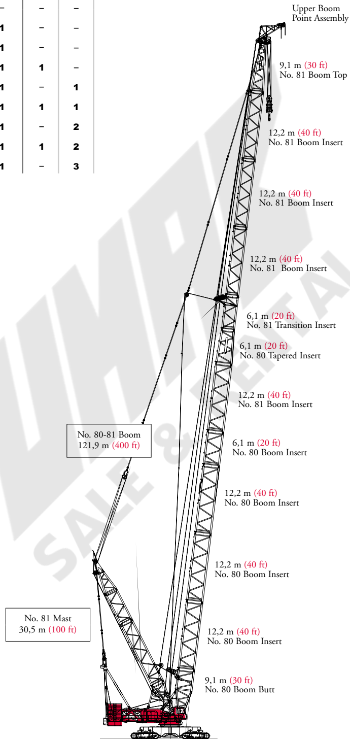
Model 21000 No. 80-81 Main Boom with No. 81 Mast 121,9 m (400 ft)
