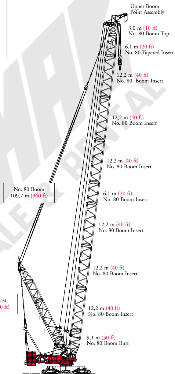
Model 21000 No. 80 Main Boom with No. 81 Mast 109,7 m (360 ft)
