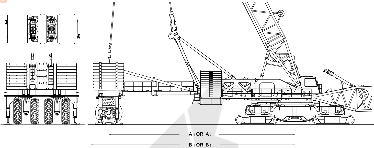
WHEELED COUNTERWEIGHT
