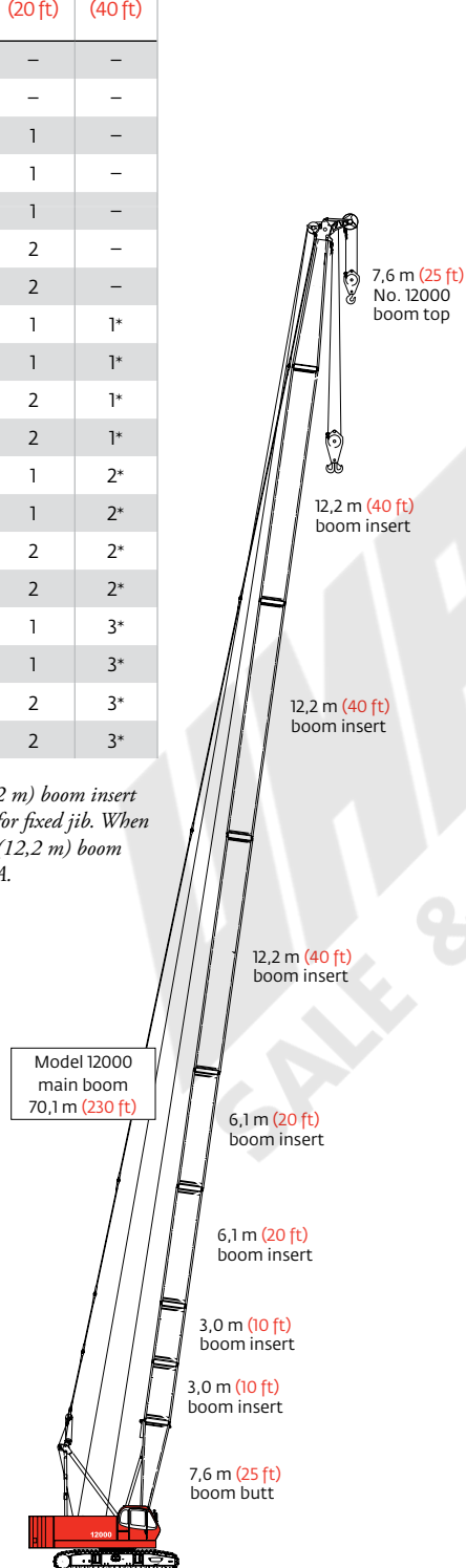
Model 12000 Main boom 70,1 m (230 ft)
