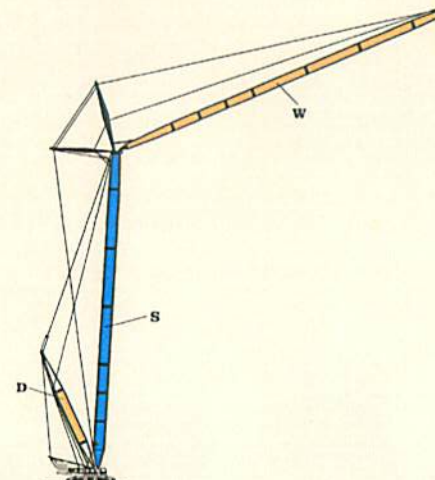
SDW 35 m - 77 m / 28 m - 84 m
