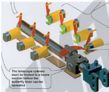
TWIN-LOCK™ Boom pinning mechanism automatically pins the sections in position using two horizontal large diameter boom pins
