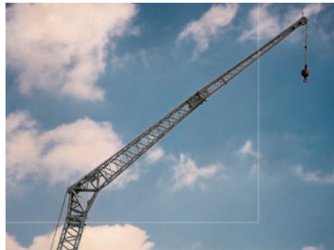
LUFFING BI-FOLD SWINGAWAY Hydraulically offset lattice bi-fold swingaway lets the operator set the offset from 0-40° while under load from the superstructure cab
