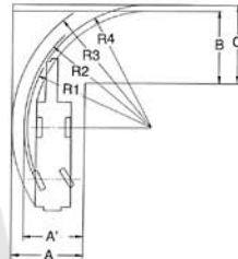
2-Drive Steering (Rear)
