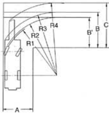
2-Drive Steering (Front)
