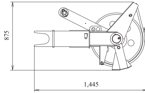
Auxiliary Sheave Weight: 340 kg
