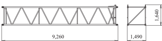
9.1 m Boom Insert with Lug Weight: 765 kg
