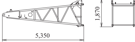
Boom Base Weight: 1,130 kg
