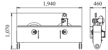
Lower Spreader (for Tower) Weight: 410 kg
