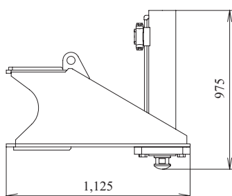
Translifter Weight: 1,220 kg / 4 pieces
