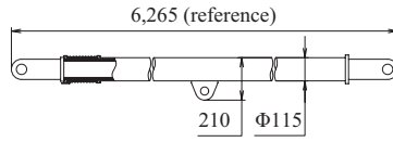
Crane Backstop Weight: 210 kg / 1 piece
