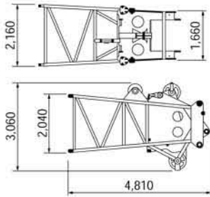
Luffing Boom Top Weight: 2,545 kg
